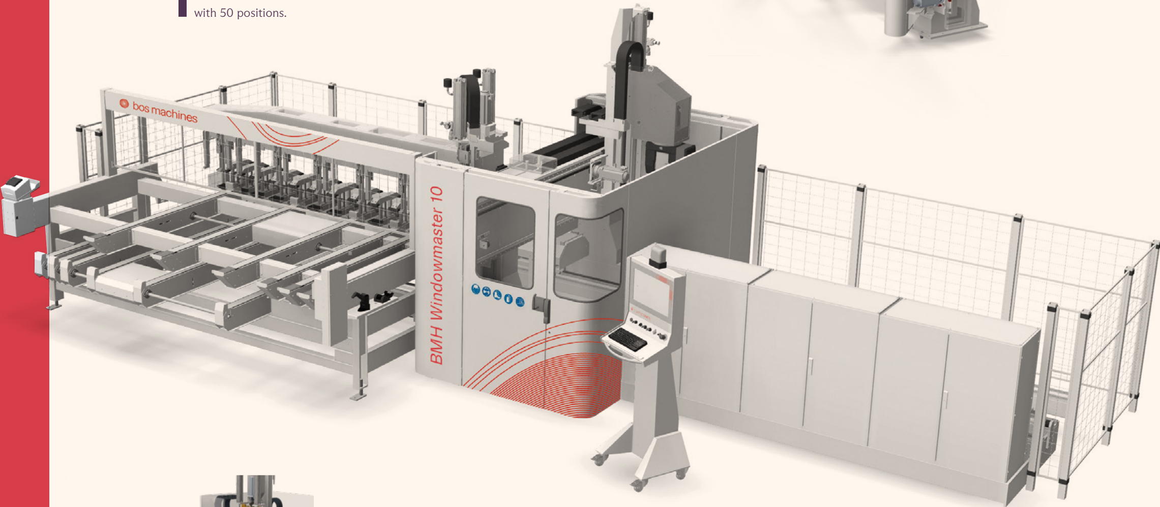
Solid gantry with 5-axis robohead and servo controlled dust hoods for optimal dust extraction.
