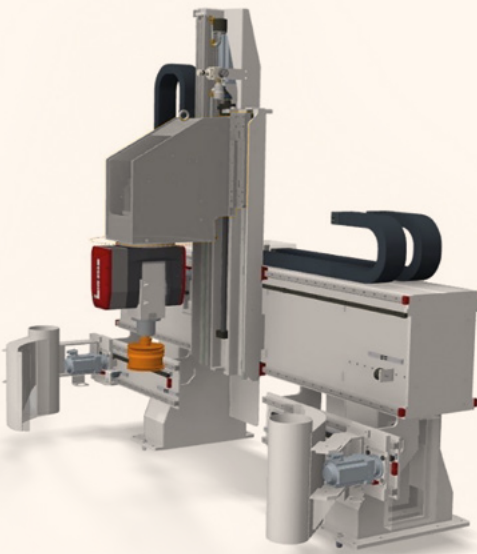
Solid gantry with 5-axis robohead and servo controlled dust hoods for optimal dust extraction.
